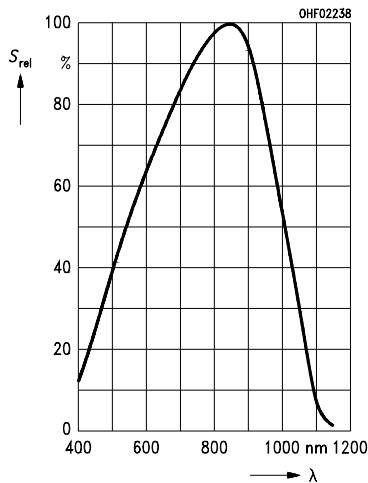
Relative Spectral Sensitivity Relative spektrale Empfindlichkeit S_{rel} = f(\lambda)
