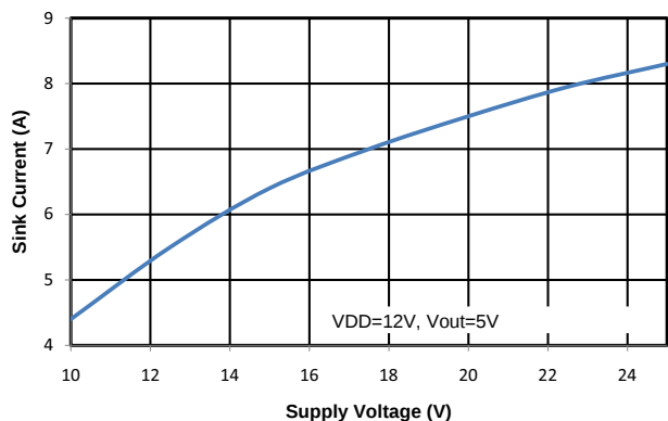
Figure 31. Output Sink Current vs. Supply Voltage
