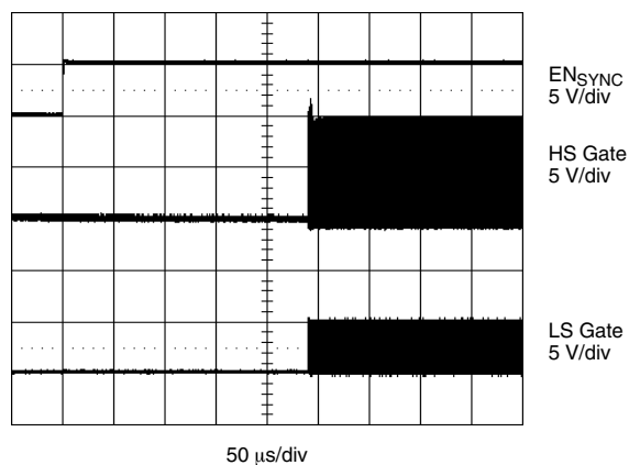
Figure 6 EN_{SYNC} Delay
