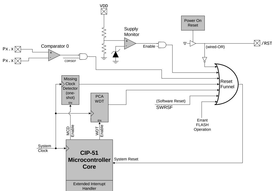
Figure 18.1. Reset Sources
