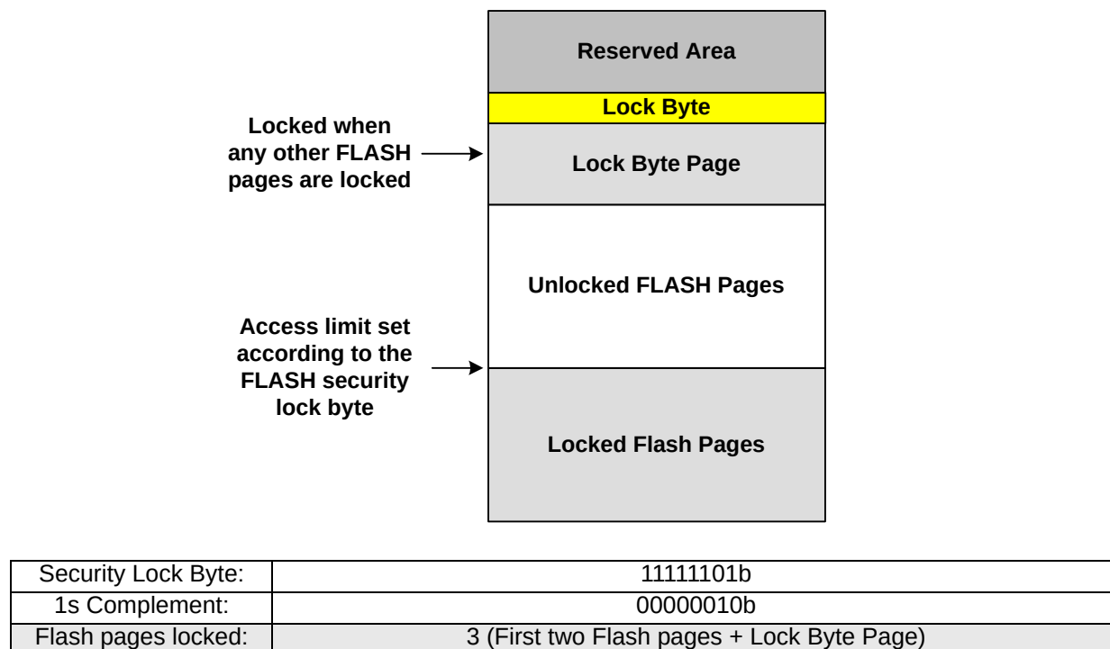
Figure 16.1. Flash Program Memory Map
