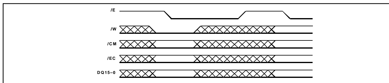
Figure 4: Write Cycle
