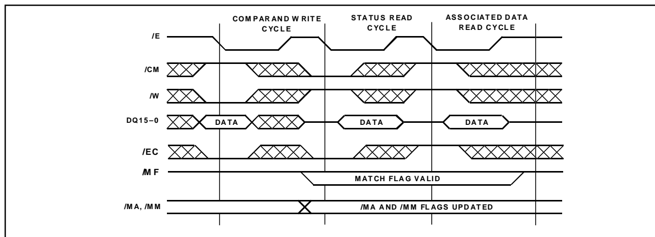
Figure 5: Cycle to Cycle Timing Example
