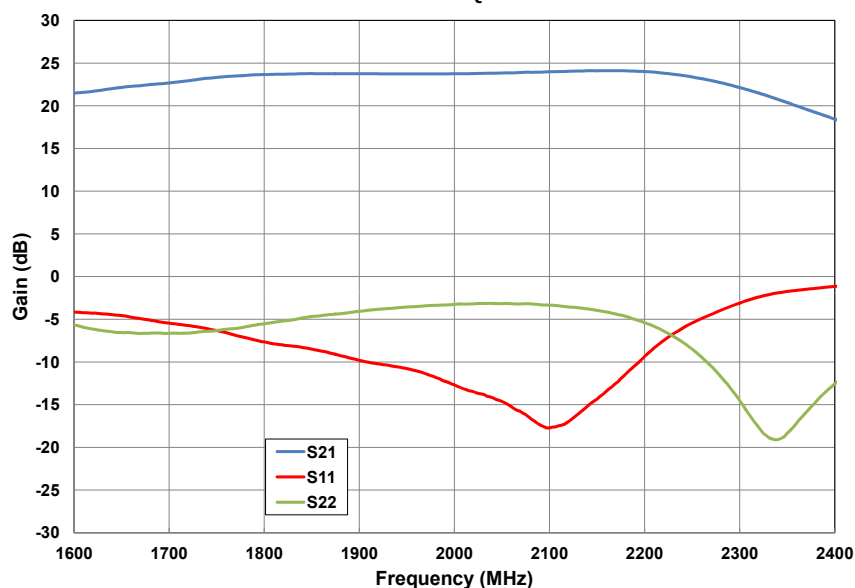
Figure 1. - Small Signal Gain and Return Losses vs Frequency for the CGHV22100 measured in CGHV22100-TB Amplifier Circuit V_{DD} = 50 \text{ V} , I_{DQ} = 0.5 \text{ A}
