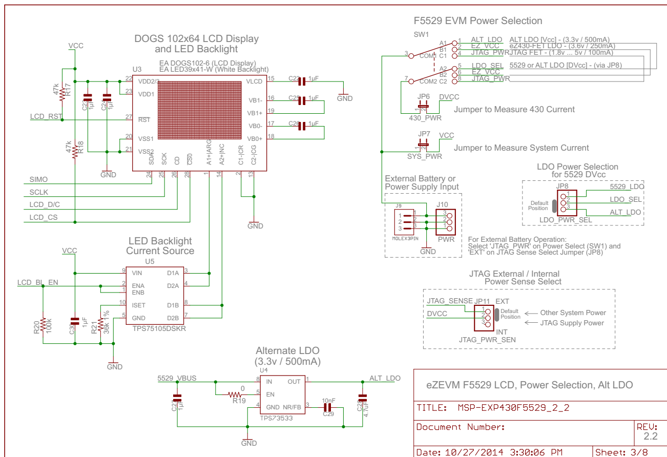
Figure 12. Schematics (3 of 8)
