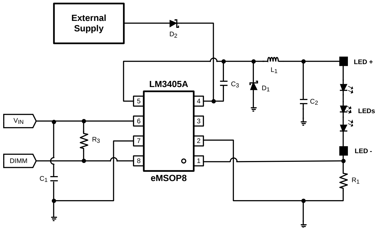
Figure 6. V_{BOOST} Derived from External Supply
