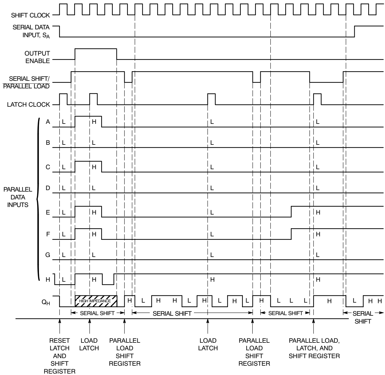
Figure 12. Timing Diagram
