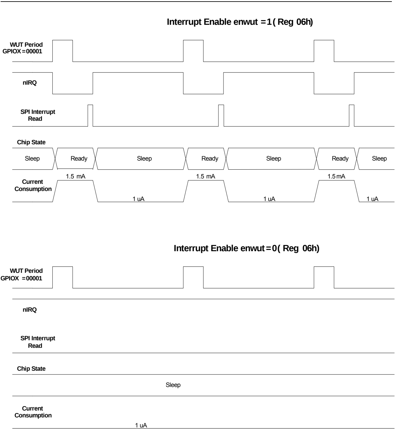
Figure 23.23. WUT Interrupt and WUT Operation
