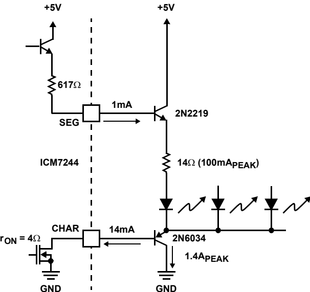
FIGURE 7A. COMMON CATHODE DISPLAY
