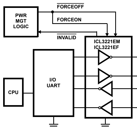
FIGURE 5. CONNECTIONS FOR MANUAL POWER-DOWN WHEN NO VALID RECEIVER SIGNALS ARE PRESENT
