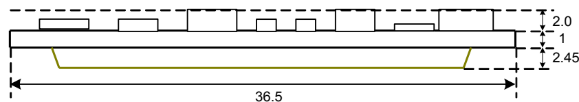
Figure 3-2: Side View with Connector mounted
