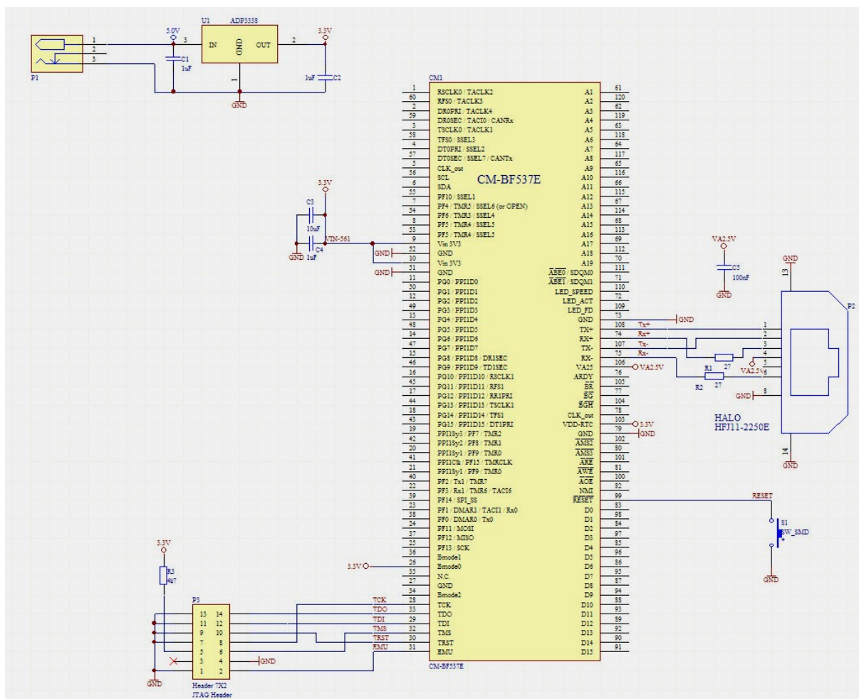
Figure 6-1: Configuration with Ethernet and JTAG Connector
