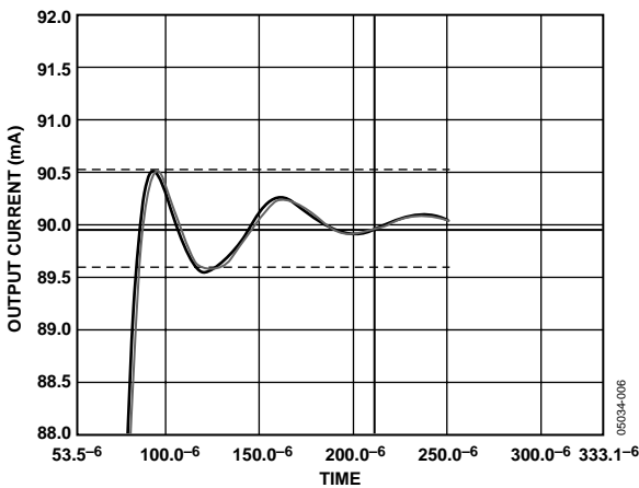
Figure 8. 1/4 to 3/4 Scale Settling Time ( V_{DD} = 3.6V )
