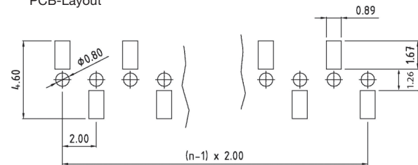
PCB-Layout
