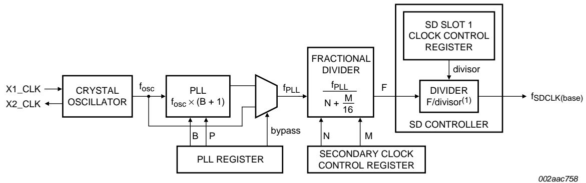
Fig 6. Secondary clock control architecture
