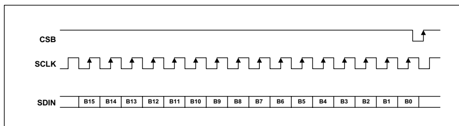
Figure 32 3-Wire Serial Interface
