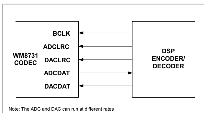
Figure 31 Slave Mode
