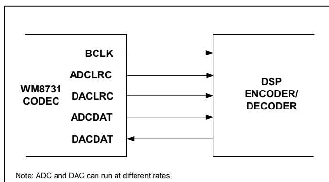
Figure 30 Master Mode
