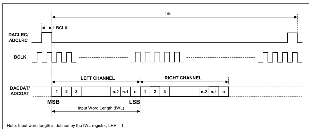
Figure 29 DSP Mode
