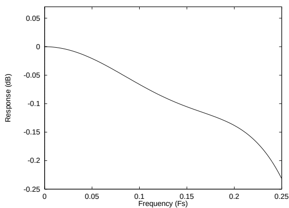
Figure 41 DAC Digital Filter Ripple –Type 3
