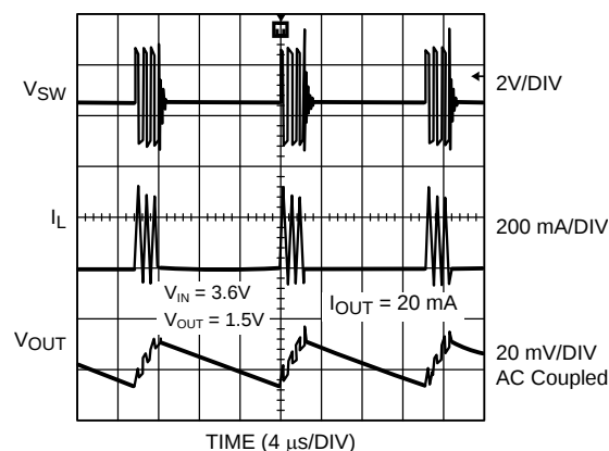
Figure 17. Typical PFM Operation
