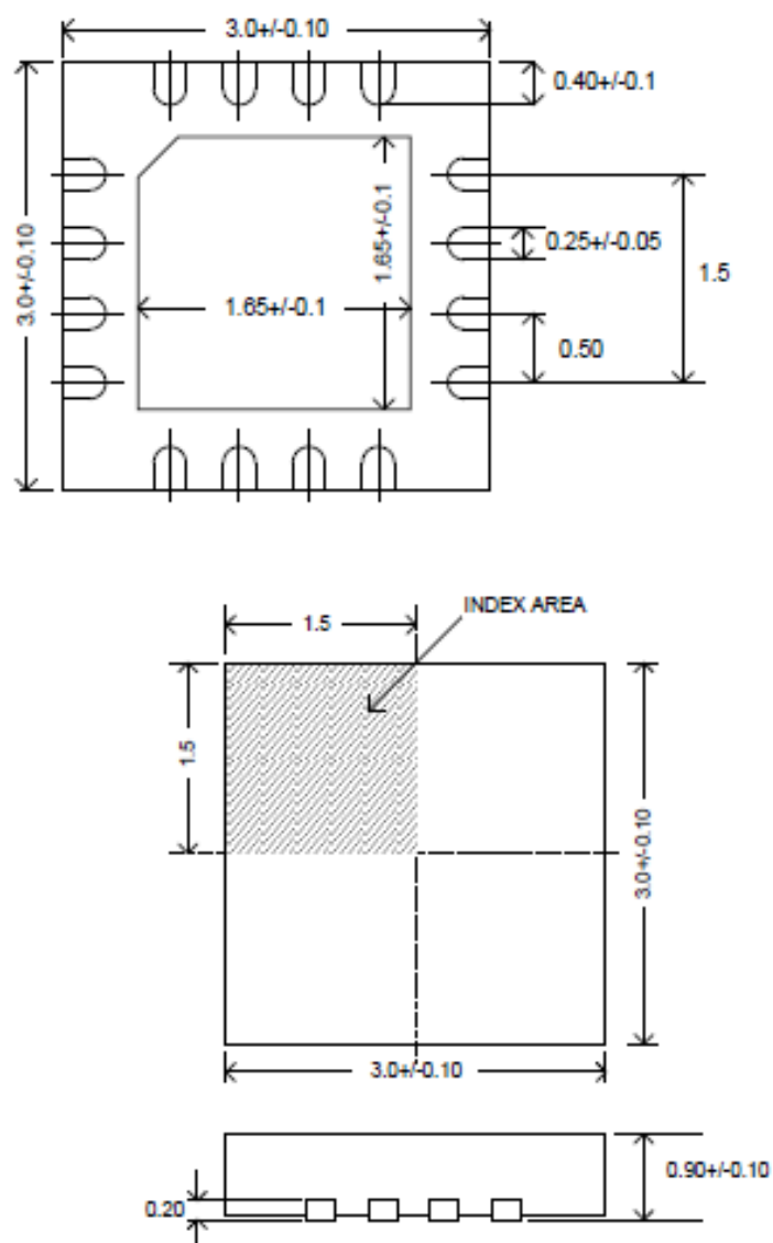
Figure 5.1: ZSPM4011 Package Drawing
