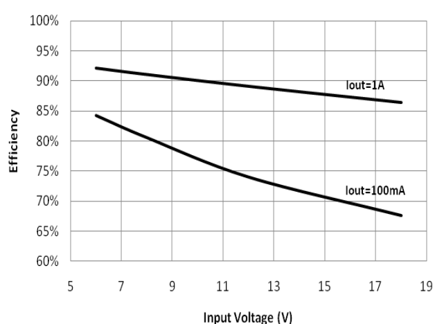
Figure 2.12: Efficiency vs. Input Voltage ( V_{OUT}=3.3V )
