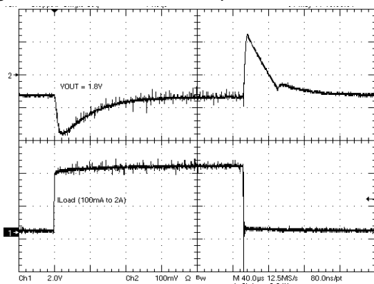
Figure 2.3: 100mA to 2A Load ( V_{CC} = 12\text{V} , V_{out} = 1.8\text{V} )
