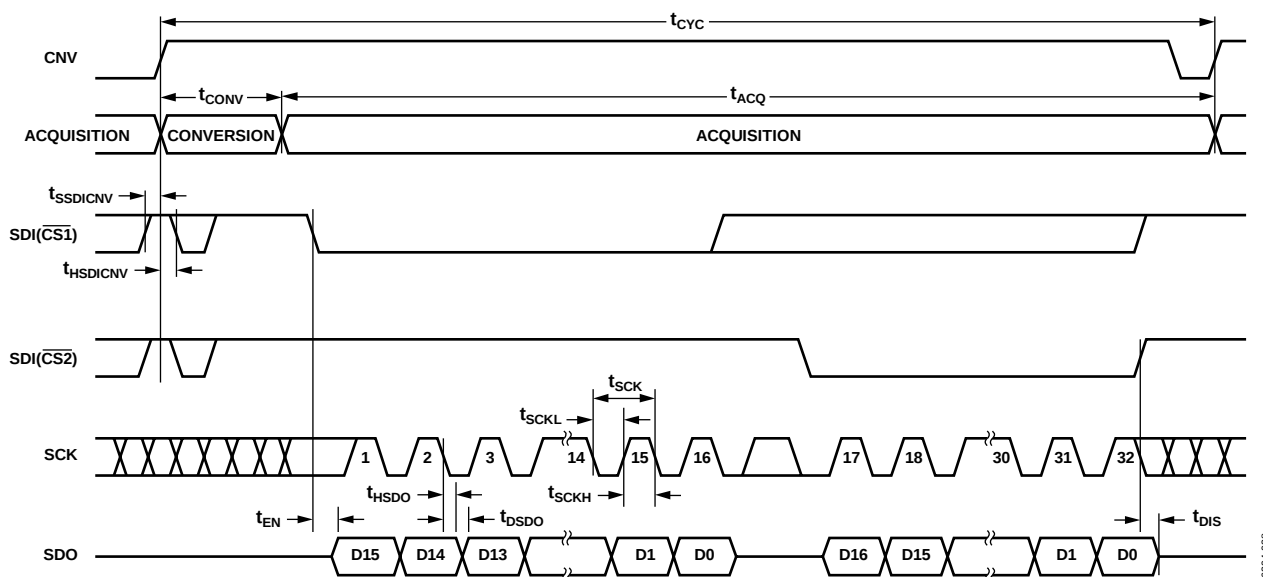
Figure 39. \overline{\text{CS}} Mode, 4-Wire Without Busy Indicator Serial Interface Timing
