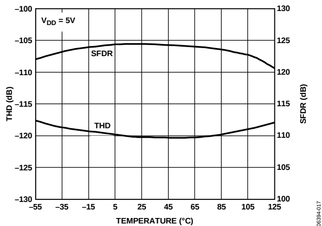
Figure 17. THD, SFDR vs. Temperature
