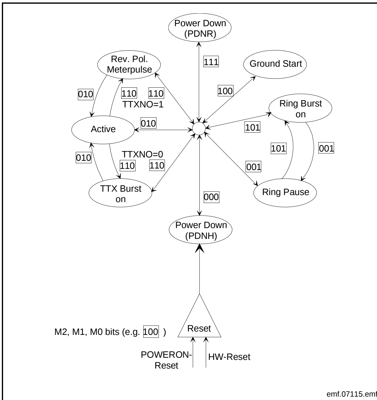
Figure 31 Operating Modes
