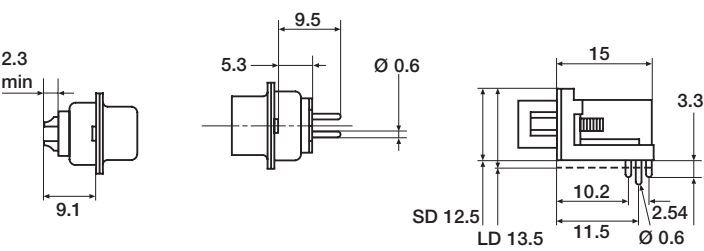
Solder Bucket Straight P. C. 90° P. C.
