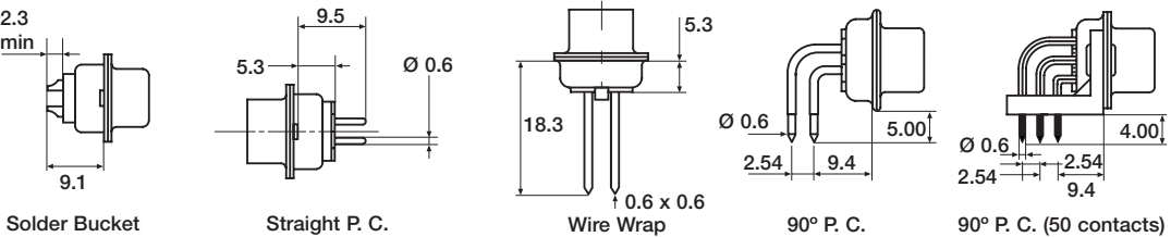
Solder Bucket Straight P. C. Wire Wrap 90° P. C. 90° P. C. (50 contacts)
