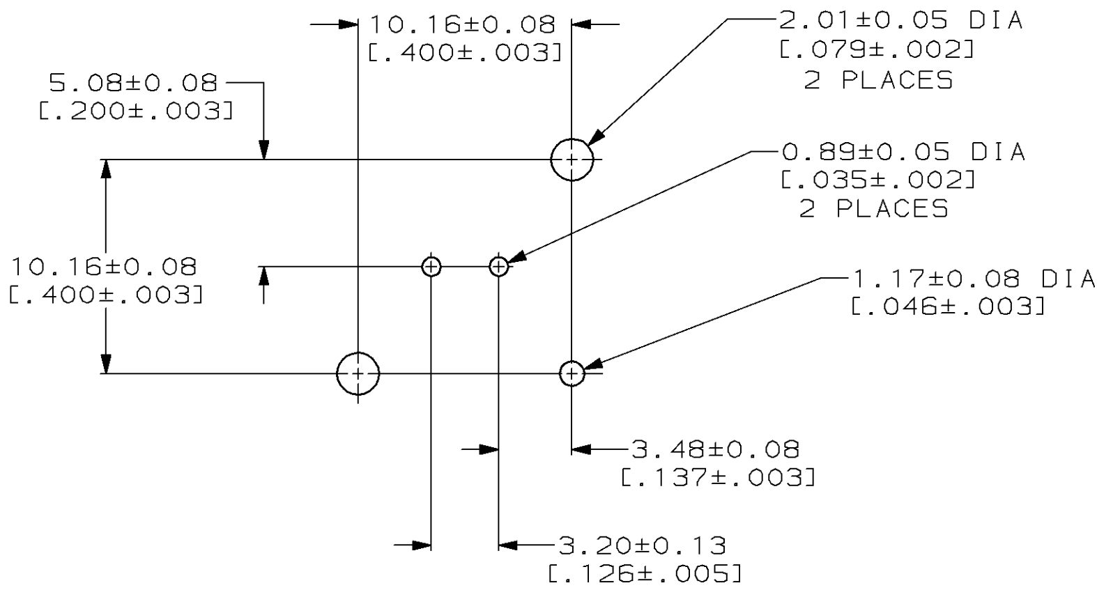
PCB CONFIGURATION
