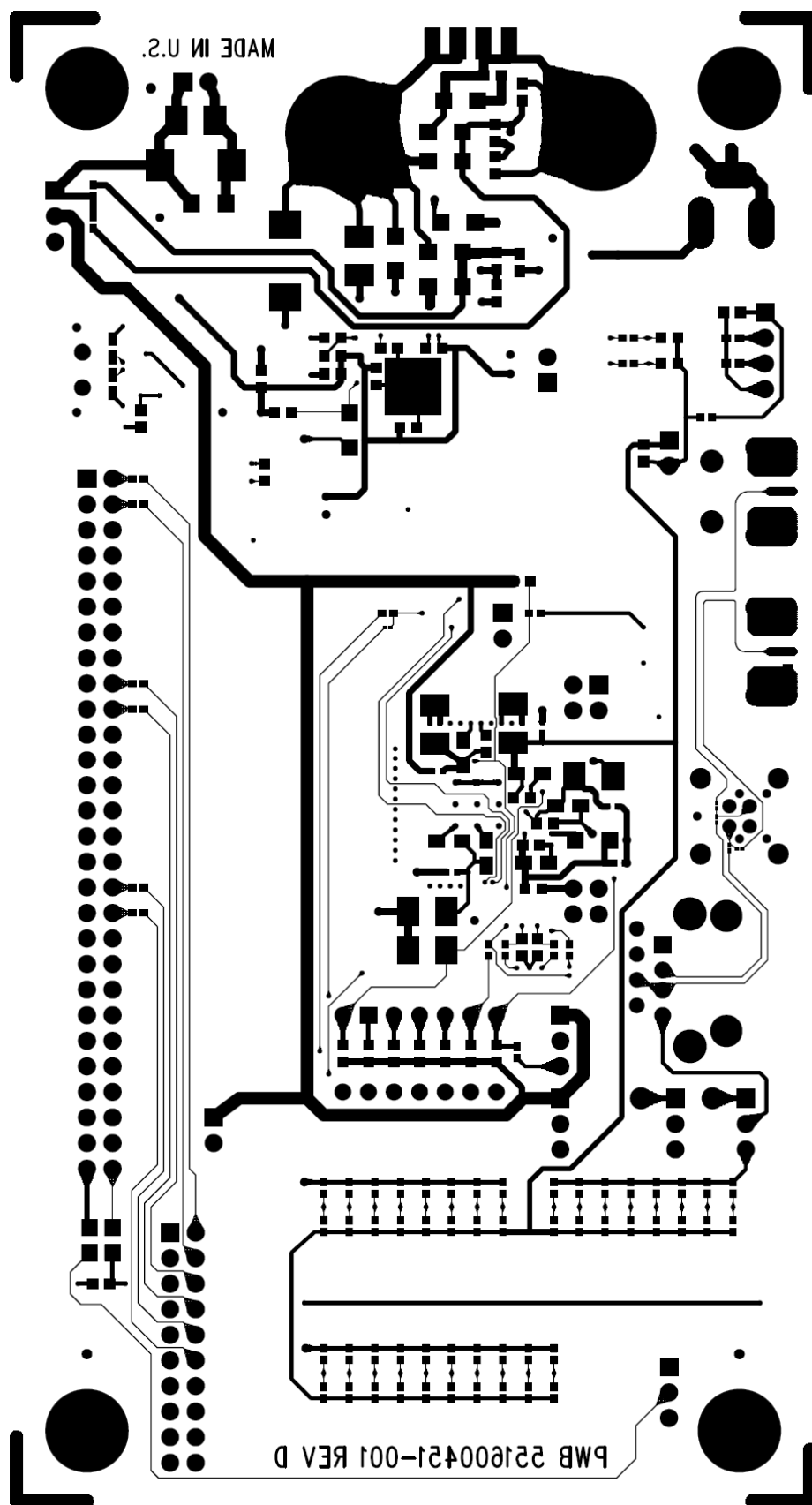
Figure 9: BOTTOM Layer
