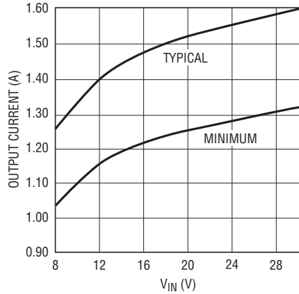
Maximum Load Current, V OUT = 5V, L = 33μH
