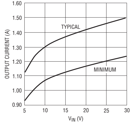
Maximum Load Current, V OUT = 3.3V, L = 4.7μH
