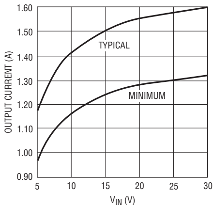
Maximum Load Current, V OUT = 3.3V, L = 10μH
