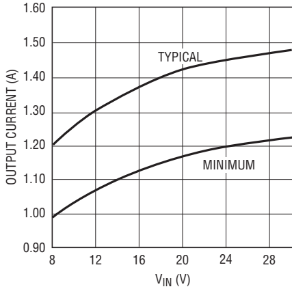
Maximum Load Current, V OUT = 5V, L = 8.2μH
