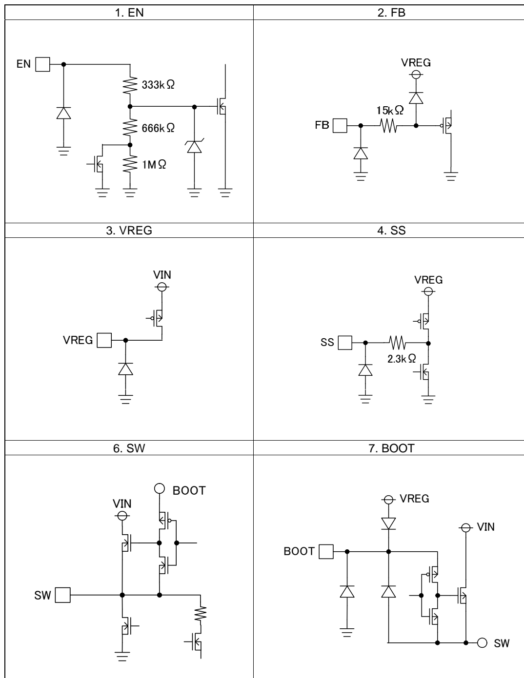
Figure 35. I/O equivalence circuit
