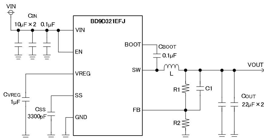
Figure 28. Application Circuit
