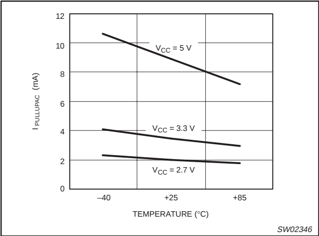
Figure 14. I PULLUPAC versus Temperature.
