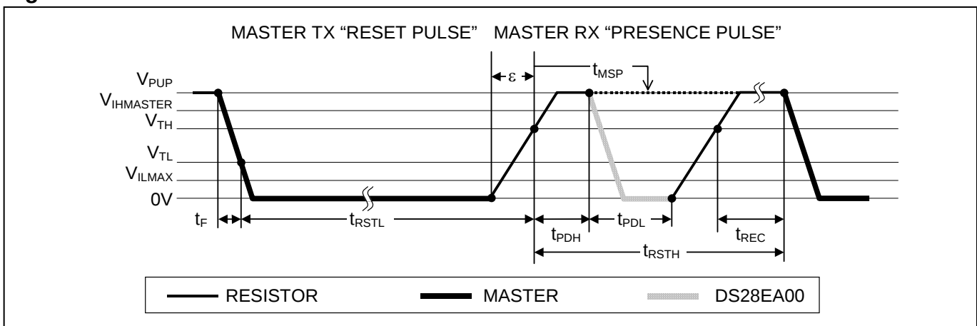
Figure 13. Initialization Procedure “Reset and Presence Pulses”
