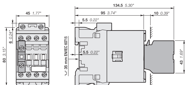
AF26, AF38 + CA4, CC4 1-pole auxiliary contact block
