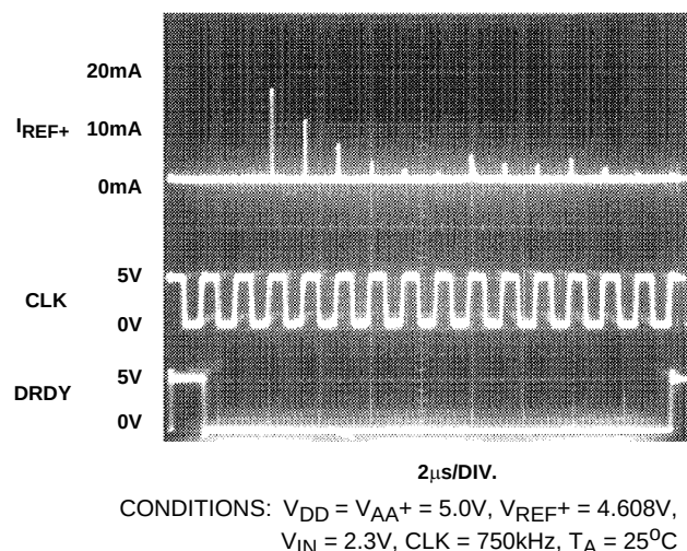
FIGURE 20. TYPICAL REFERENCE INPUT CURRENT
