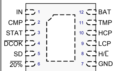
LD Package (Top View)
