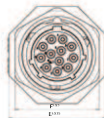
MATING FACE
