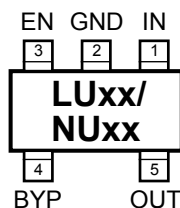
MIC5247-x.xBM5 / YM5 MIC5247-x.xBD5 / YD5 (Top View)
