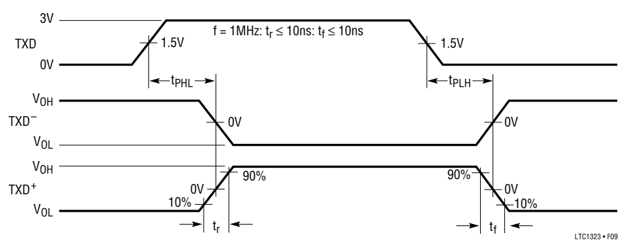
Figure 9. Differential Driver With Single-Ended Load
