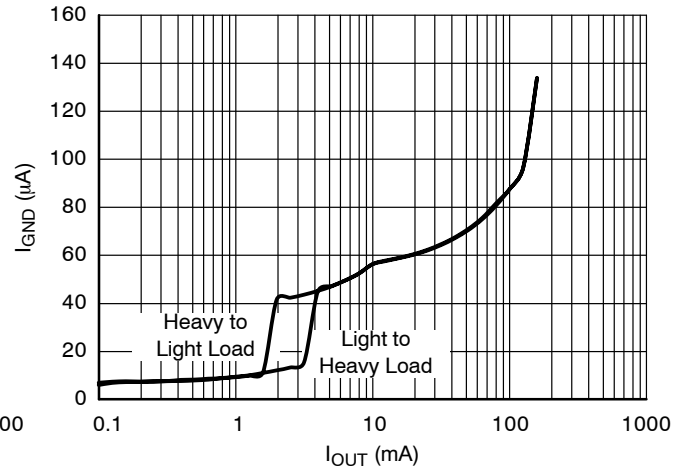
Figure 14. Supply Current vs. Output Current, 2.8 V Version, V_{IN} = 3.8 V, V_{AE} = 0 V
