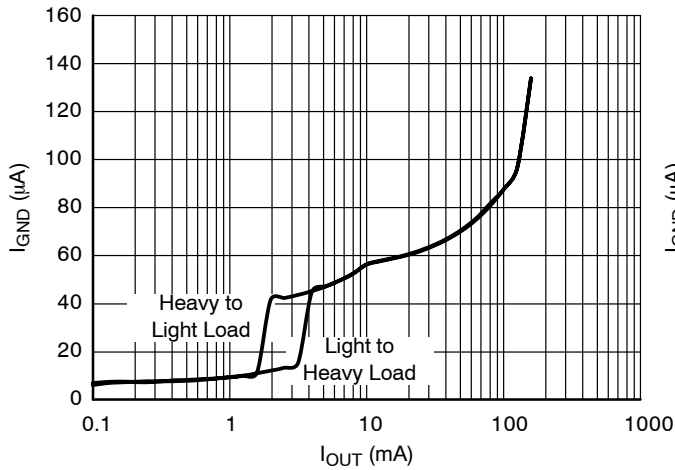
Figure 13. Supply Current vs. Output Current, 1.2 V Version, V_{IN} = 2.2 V, V_{AE} = 0 V
