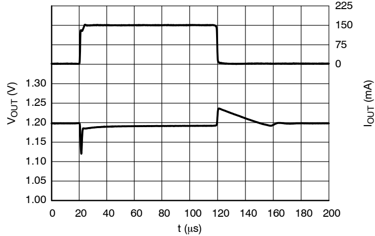
Figure 29. Load Transients, 1.2 V Version, I_{OUT} = 1 - 150 \text{ mA} , t_R = t_F = 0.5 \text{ } \mu\text{s} , V_{IN} = 2.2 \text{ V} , AE = V_{IN} \text{ V}
