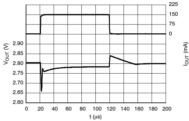
Figure 28. Load Transients, 2.8 V Version, I_{OUT} = 1 - 150 \text{ mA} , t_R = t_F = 0.5 \text{ } \mu\text{s} , V_{IN} = 2.2 \text{ V} , AE = 0 \text{ V}
