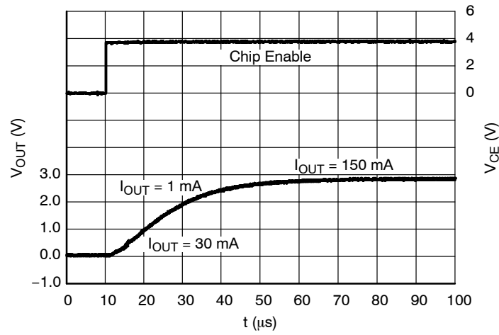
Figure 40. Start-up, 2.8 V Version, V_{IN} = 3.8\text{ V}
