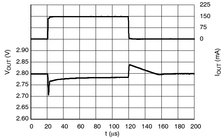
Figure 30. Load Transients, 2.8 V Version, I_{OUT} = 1 - 150 \text{ mA} , t_R = t_F = 0.5 \text{ } \mu\text{s} , V_{IN} = 2.8 \text{ V} , AE = V_{IN} \text{ V}
