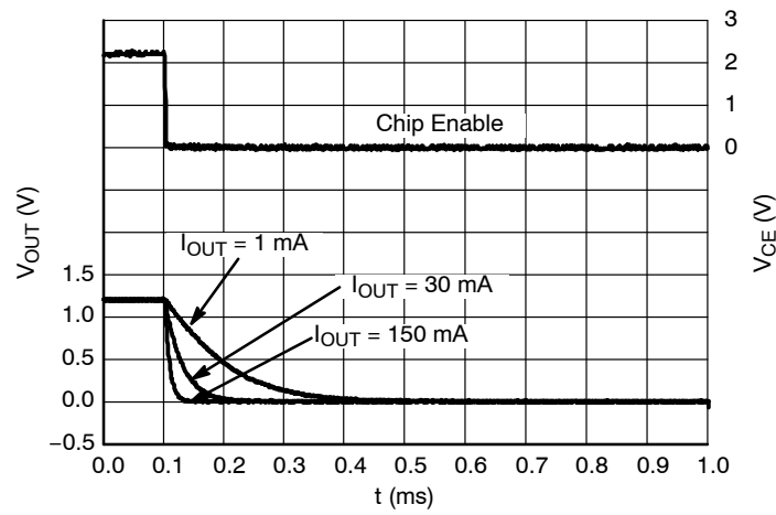
Figure 41. Shutdown, 1.2 V Version, V_{IN} = 2.2\text{ V}
