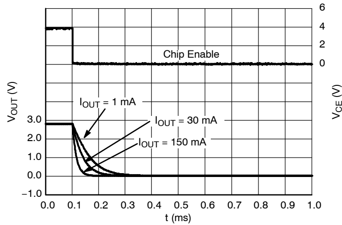
Figure 42. Shutdown, 2.8 V Version, V_{IN} = 3.8\text{ V}
