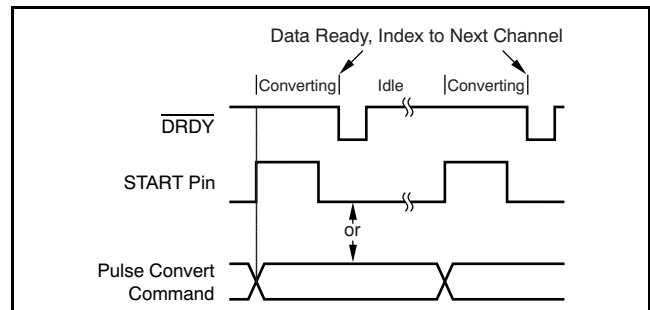
Figure 41. Pulse Conversion, Auto-Scan Mode
