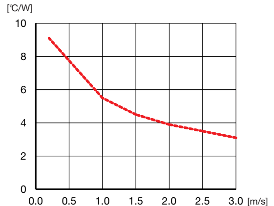
Thermal resistance vs. airspeed measured at the converter. Tested in windtunnel with airflow and test conditions as per the Thermal consideration section.
