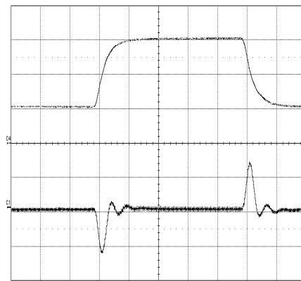
Output voltage response to load current step-change (5-15-5 A) at T_{Pcb}=+25\text{ }^{\circ}C , V_{in}=53\text{ V} . Top trace: load current (5 A/div.). Bottom trace: output voltage (100mV/div.) Time scale: 0.1 ms/div.
