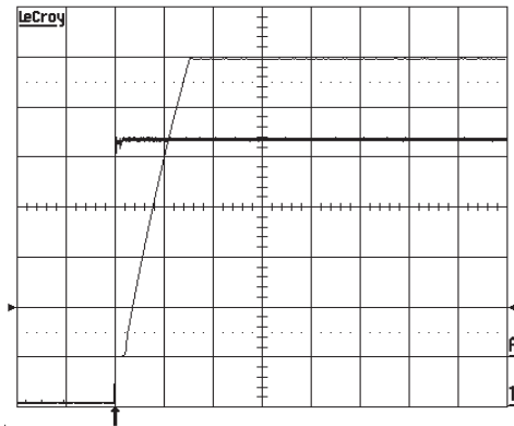
Start-up at I_o=4.2 A resistive load at T_{Pcb}=+25 °C, V_{in}=53 V. Start enabled by connecting V_{in} . Top trace: output voltage (2 V/div.). Time scale: 5 ms/div. Bottom trace: input voltage (10 V/div.).
