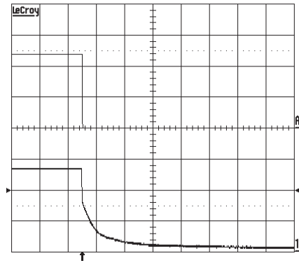
Turn-off at I_o=4.2 A resistive load at T_{Pcb}=+25 °C, V_{in}=53 V. Turn-off enabled by disconnecting V_{in} . Top trace: output voltage (5 V/div.). Bottom trace: input voltage (20 V/div.). Time scale: 10 ms/div.
