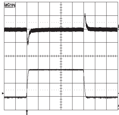
Output voltage response to load current step-change (1.05-3.15-1.05 A) at T_{Pcb}=+25 °C, V_{in}=53 V. Top trace: output voltage (200mV/div.). Bottom trace: load current (1 A/div.) Time scale: 0.1 ms/div.
