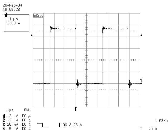
FIGURE 14. FET DRAIN-SOURCE VOLTAGE
