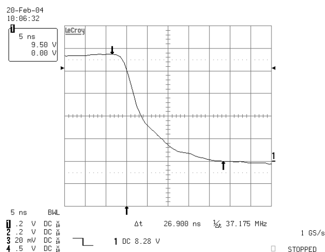
FIGURE 15. FET D-S VOLTAGE NEAR-ZVS TRANSITION
