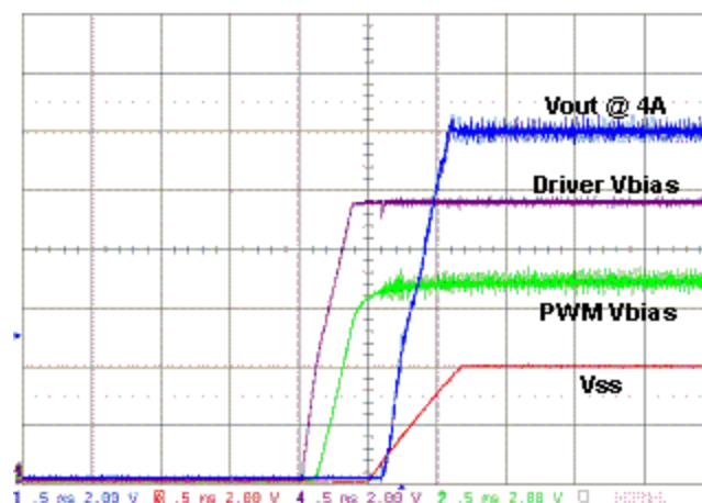
FIGURE 17. OUTPUT SOFT-START
