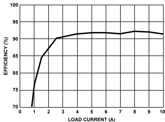
FIGURE 10. EFFICIENCY vs LOAD V_{IN} = 48V
