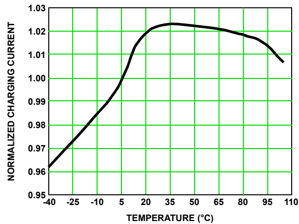
FIGURE 4. CHARGE CURRENT vs TEMPERATURE
