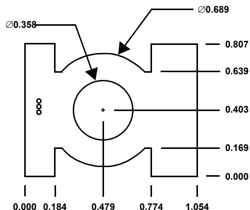
FIGURE 7G. PWB DIMENSIONS
