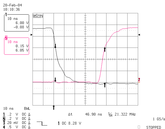
FIGURE 16. OUTA - OUTB TRANSITION
