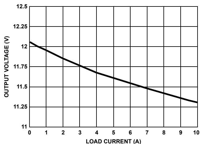
FIGURE 11. LOAD REGULATION AT V_{IN} = 48V
