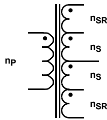
FIGURE 6. TRANSFORMER SCHEMATIC
