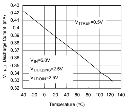
V_{TTREF} Discharge Current vs Temperature
