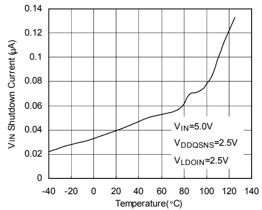
V_{IN} Shutdown Current vs Temperature
