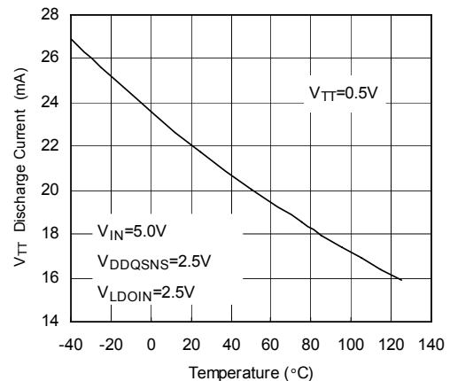
V_{TT} Discharge Current vs Temperature
