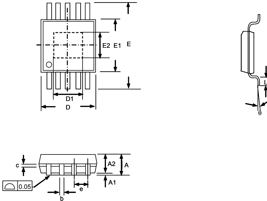
MSOP-10 (FD) Package
