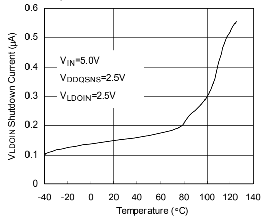
V_{LDOIN} Shutdown Current vs Temperature
