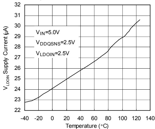
V_{LDOIN} Supply Current vs Temperature
