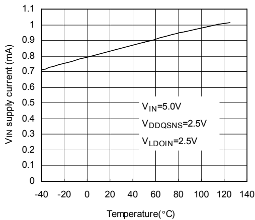
V_{IN} Supply Current vs Temperature
