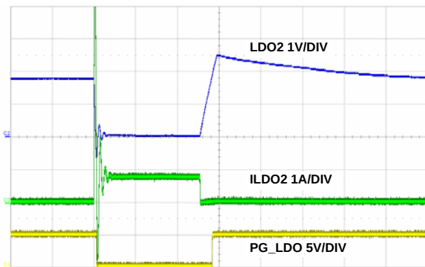
FIGURE 30. LDO2 SHORT CIRCUIT AND RECOVERY, 200µs/DIV
