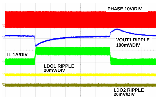
FIGURE 21. LOAD TRANSIENT, 200µs/DIV
