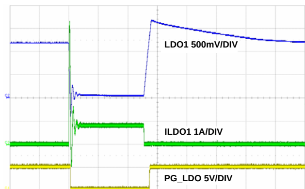
FIGURE 29. LDO1 SHORT CIRCUIT AND RECOVERY, 200µs/DIV
