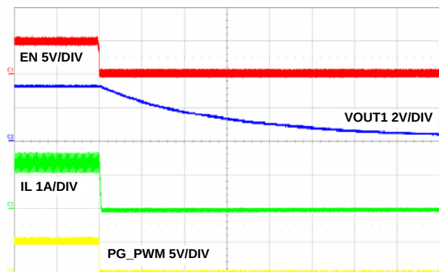
FIGURE 25. SHUT DOWN CIRCUIT AT FULL LOAD, 100µs/DIV
