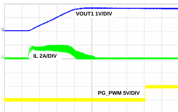
FIGURE 28. OUTPUT SHORT CIRCUIT RECOVERY, 200µs/DIV
