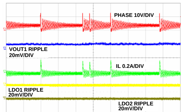
FIGURE 19. STEADY STATE OPERATION AT NO LOAD, 5 \mu s/DIV
