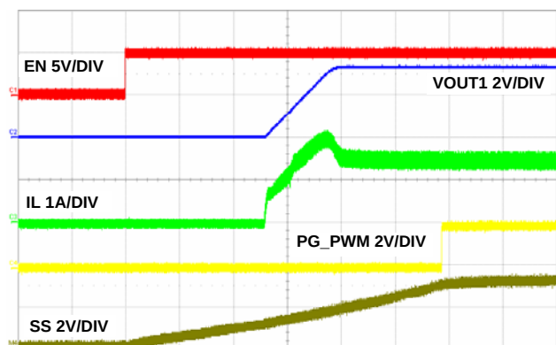
FIGURE 23. SOFT-START AT FULL LOAD, 500µs/DIV
