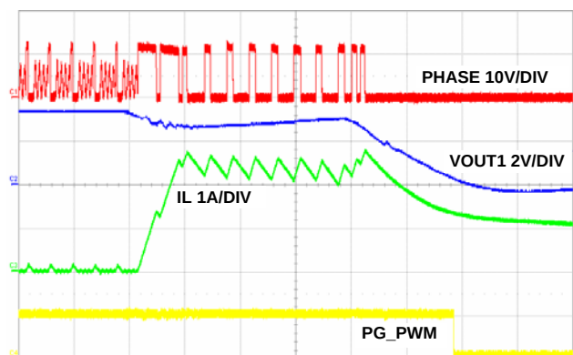
FIGURE 27. OUTPUT SHORT CIRCUIT, 5µs/DIV
