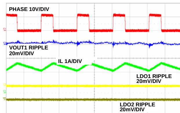
FIGURE 20. STEADY STATE OPERATION AT FULL LOAD, 1 \mu s/DIV
