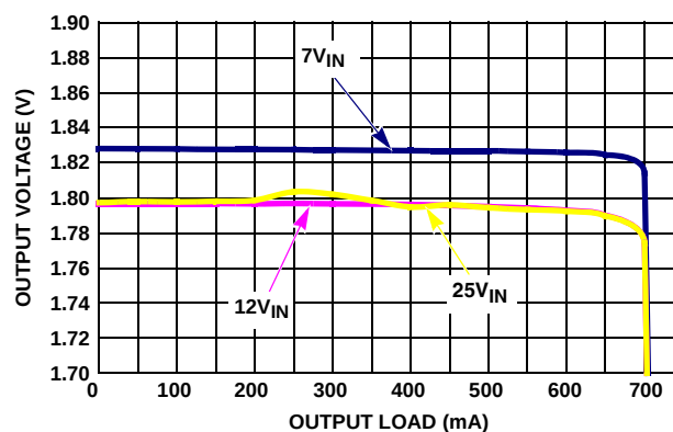
FIGURE 18. LDO2 vs LOAD, 500kHz V_{IN\_LDO2} = 3.3V
