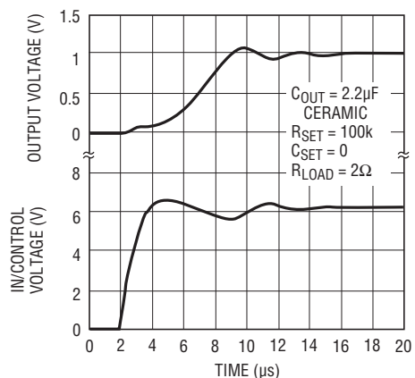
Turn-On Response
