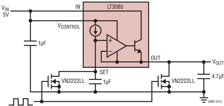
Ramp Generator
