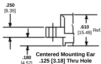
Centered Mounting Ear .125 [3.18] Thru Hole
