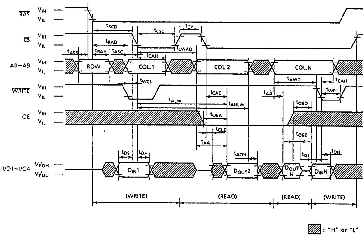
STATIC COLUMN MODE READ/WRITE MIXED CYCLE
