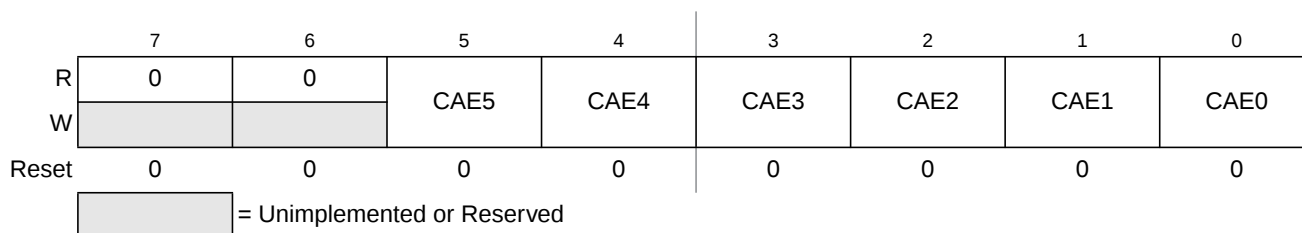
Figure 10-7. PWM Center Align Enable Register (PWMCAL)
