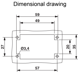
Mounting cutout when used without housing
