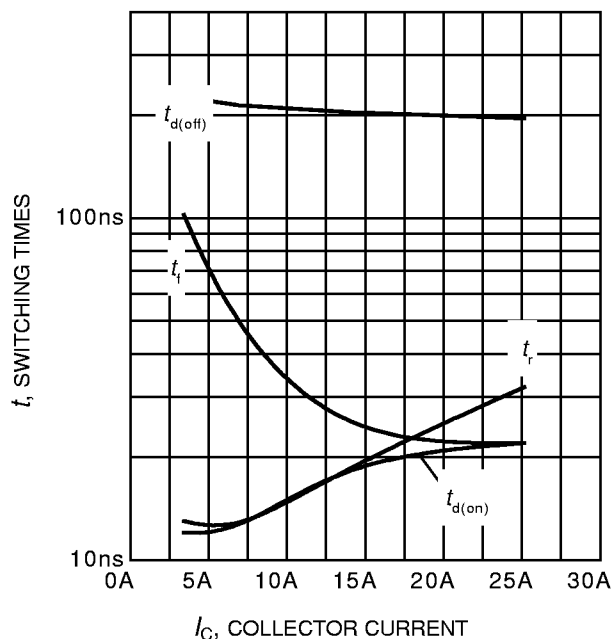
Figure 9. Typical switching times as a function of collector current (inductive load, T_j = 150^\circ\text{C} , V_{CE} = 600\text{V} , V_{GE} = -15\text{V}/+15\text{V} , R_G = 47\Omega )
