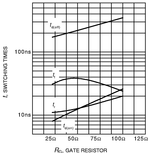
Figure 10. Typical switching times as a function of gate resistor (inductive load, T_j = 150^\circ\text{C} , V_{CE} = 600\text{V} , V_{GE} = -15\text{V}/+15\text{V} , I_C = 7\text{A} )
