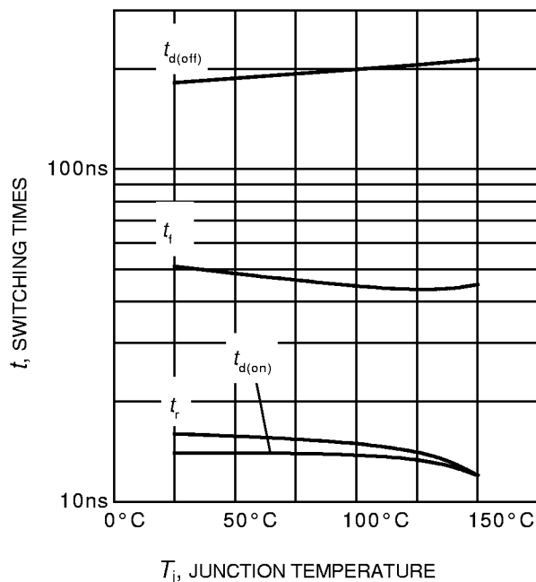
Figure 11. Typical switching times as a function of junction temperature (inductive load, V_{CE} = 600\text{V} , V_{GE} = -15\text{V}/+15\text{V} , I_C = 7\text{A} , R_G = 47\Omega )
