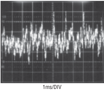
LT1761-5 10Hz to 100kHz Output Noise C_{\text{BYP}} = 100\text{pF}
