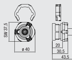
Erdkontakt Stift Contact for grounding male
