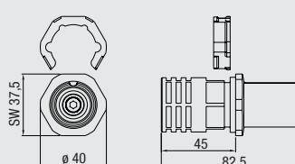
Powerkontakt Buchse Contact for power female
