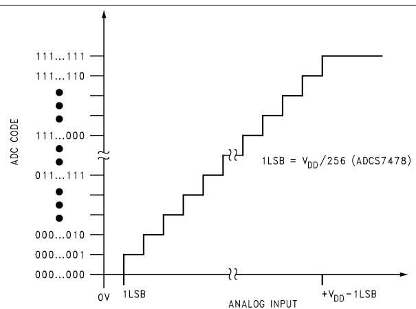
Figure 34. ADCS7478 Ideal Transfer Characteristic
