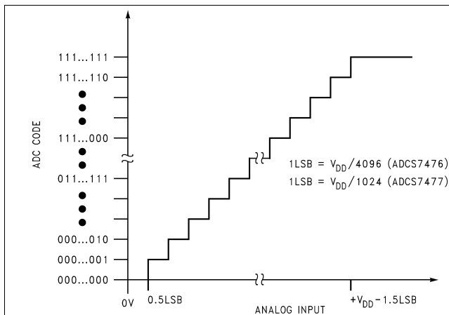
Figure 33. ADCS7476/77 Ideal Transfer Characteristic
