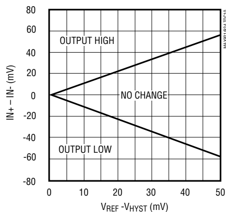
HYSTERESIS CONTROL
