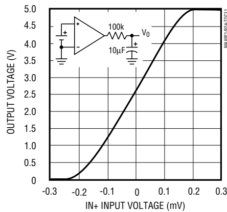
TRANSFER FUNCTION
